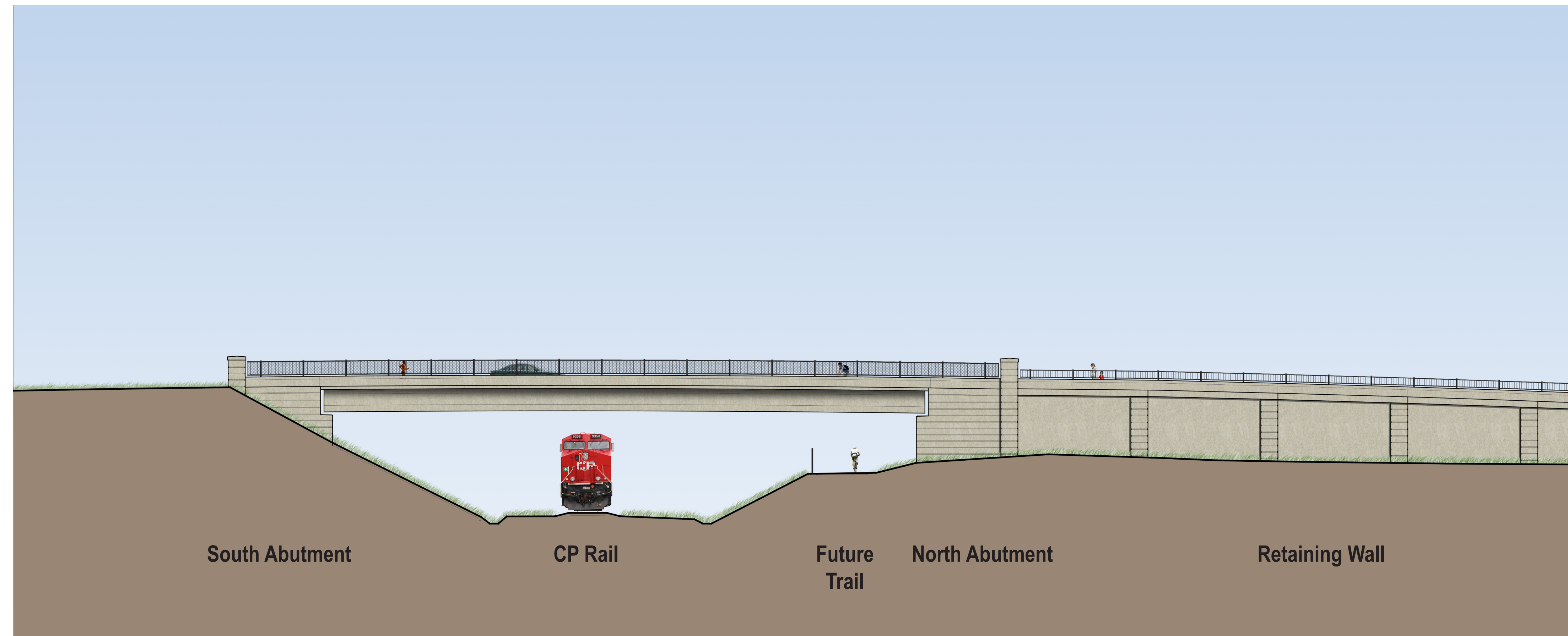
View of Full Bridge Looking West
