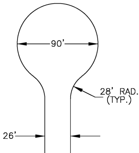
90' DIAMETER CUL-DE-SAC PERMANENT
