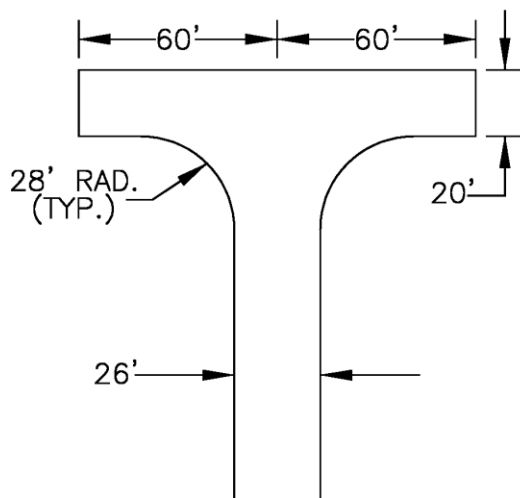
120' HAMMERHEAD TEMPORARY
