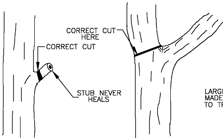
UPRIGHT BRANCH
